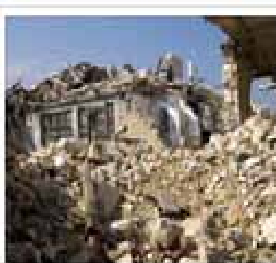
Earthquakes
